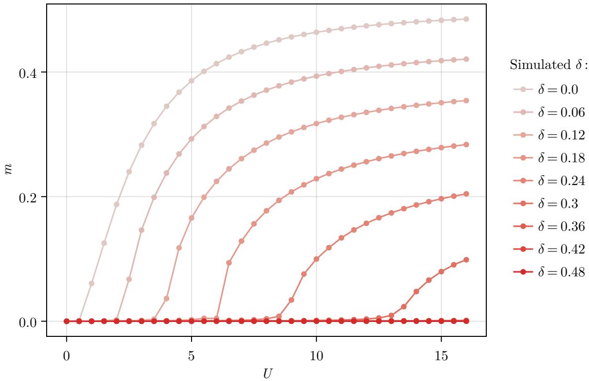
Magnetization ( t = 1.0 , V = 0.0 , L = 256 , \beta = 100.0 )
